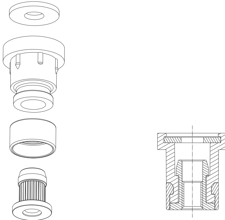
SITEC® Rivet HT for high temperatures – exploded view
