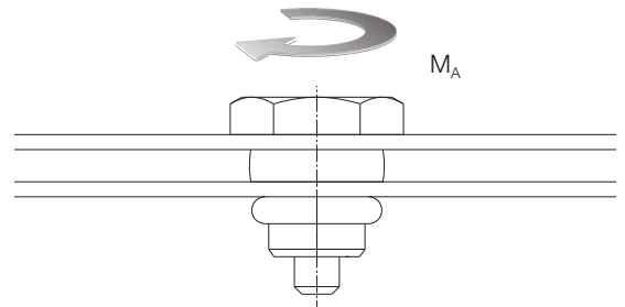
Test method to determine the torque on the SITEC® Rivet with washer
