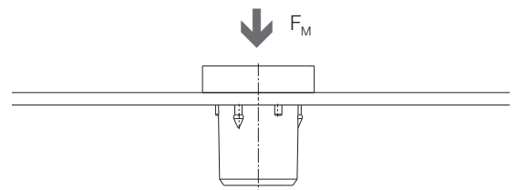
Test method to determine the installation force prior to setting
